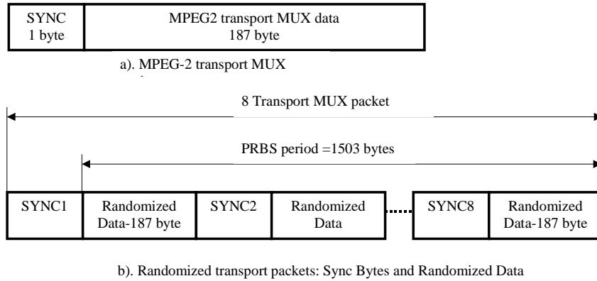
Fig.2. Packet structure in DVB
