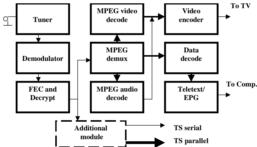
Fig. 3. Block diagram of DVB receiver
