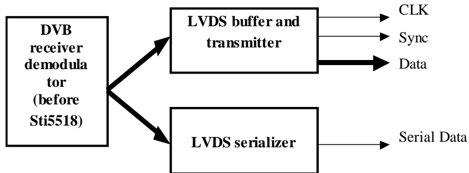
Fig. 4. Block diagram of the additional module
