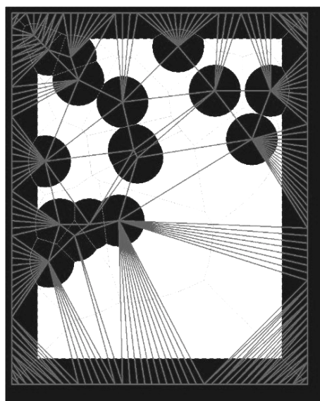
Fig. 1. Initial environment: circular obstacles, Delaunay triangulation, Voronoi diagrams
