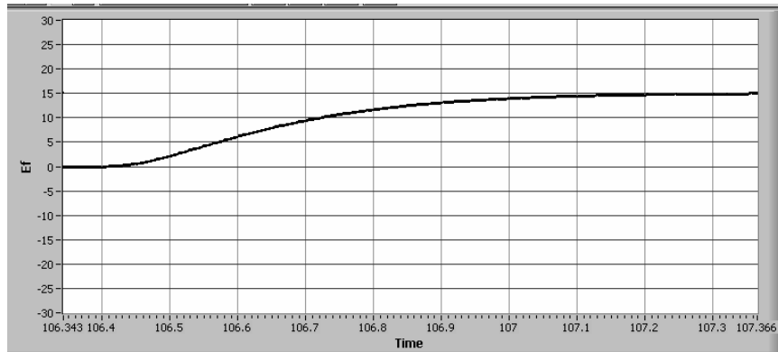
Fig.4 Response of the exciter for a step decrease of 15% of bus bar voltage
