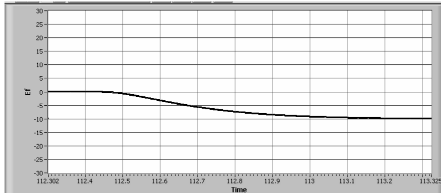
Fig.5 Response of the exciter for a step increase of 10% of bus bar voltage
