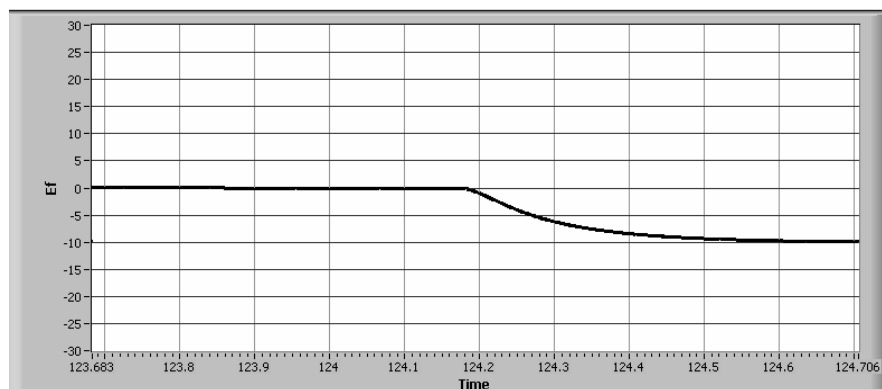
Fig.6 Response of the exciter for a step increase of 10% of bus bar voltage, modified coefficients
